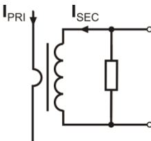
44 Fig. 16. Current transformer clamp with voltage output.
